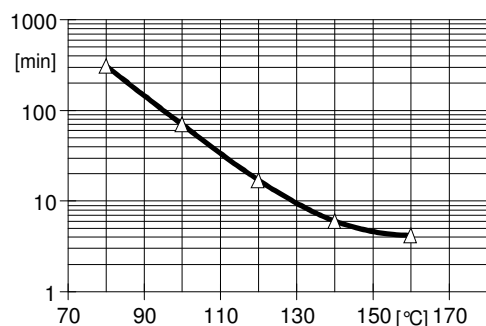
Fig. 4.3: Gelttime measured as a function of temperature (measurements with Gelnorm Instrument / ISO 9396)
