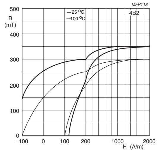
Fig.3 Typical B-H loops.
