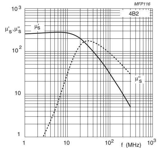
Fig.1 Complex permeability as a function of frequency.
