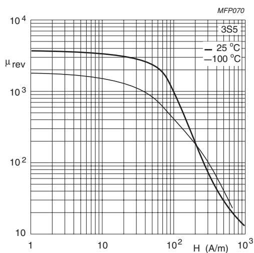
Fig.2 Reversible permeability as a function of magnetic field strength.
