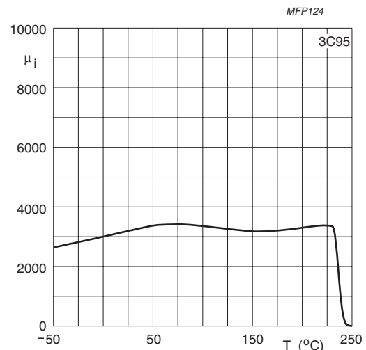
Fig.1 Initial permeability as a function of temperature.
