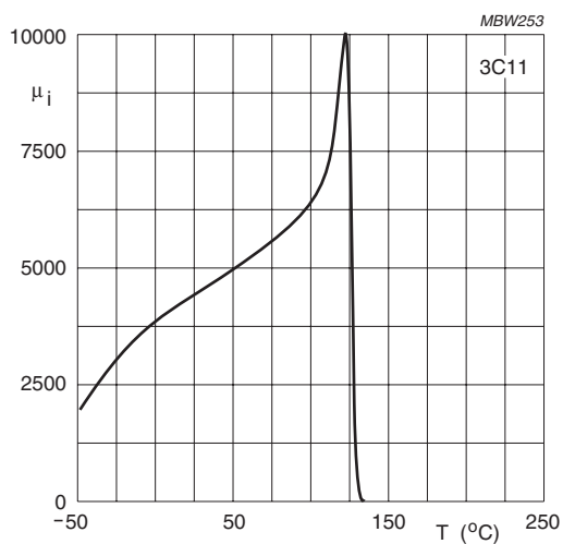
Fig.2 Initial permeability as a function of temperature.
